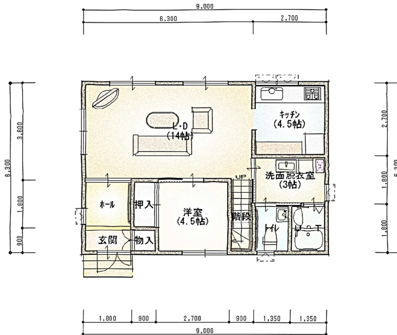
First floor plan 1 階
